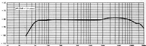
Nominal frequency response
