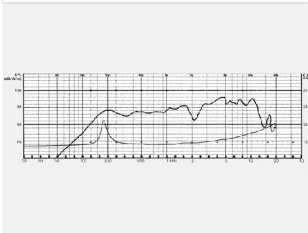
frequency response
