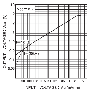
Fig. 3 Output voltage vs. input voltage
