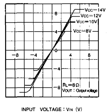
Fig. 3 I/O characteristics (variable supply voltage)
