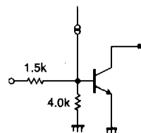
Fig. 7 A mute pin
