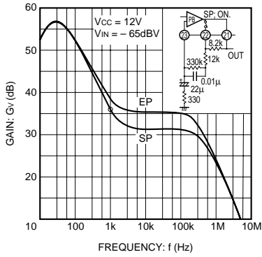
Fig. 4 Gain vs. frequency (PB amplifier)
