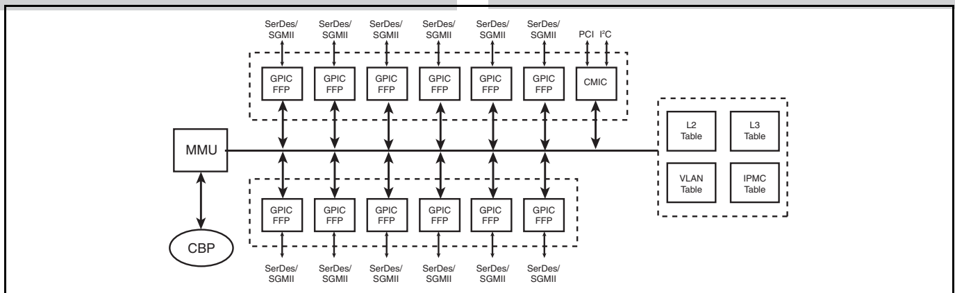
12-Port Gigabit Ethernet Multilayer Switch
