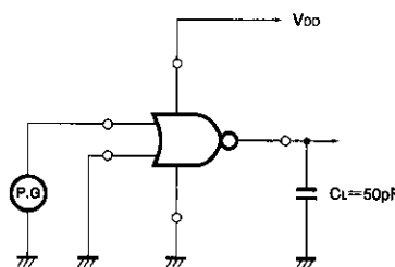
Fig.2 Switching characteristics measurement circuit
