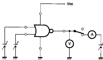
Fig.1 DC characteristics measurement circuit
