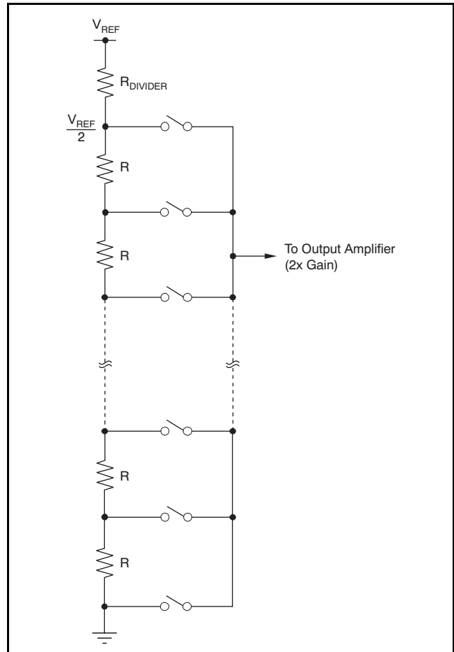
Figure 121. Resistor String
