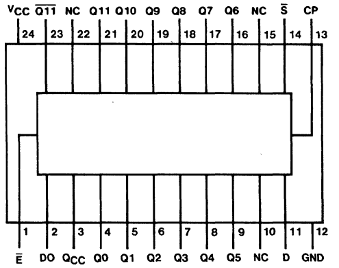
Dual-In-Line Package
