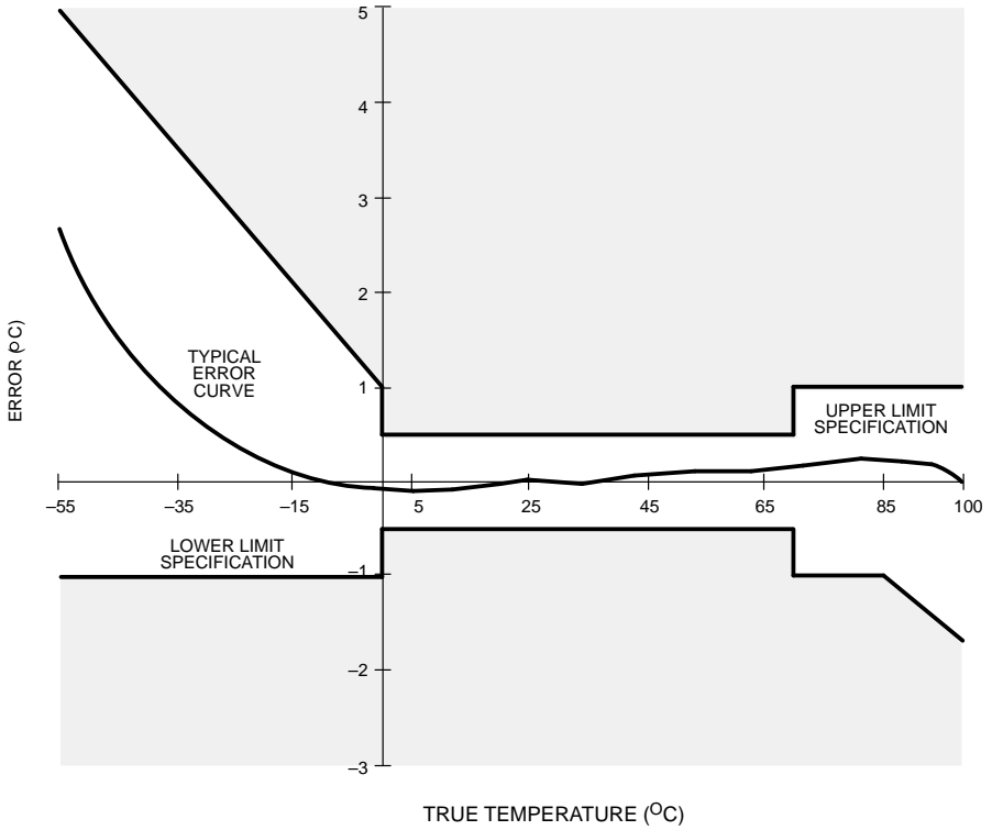
DS1920 TEMPERATURE iButton TEMPERATURE READING ERROR AND TOLERANCE BAND
