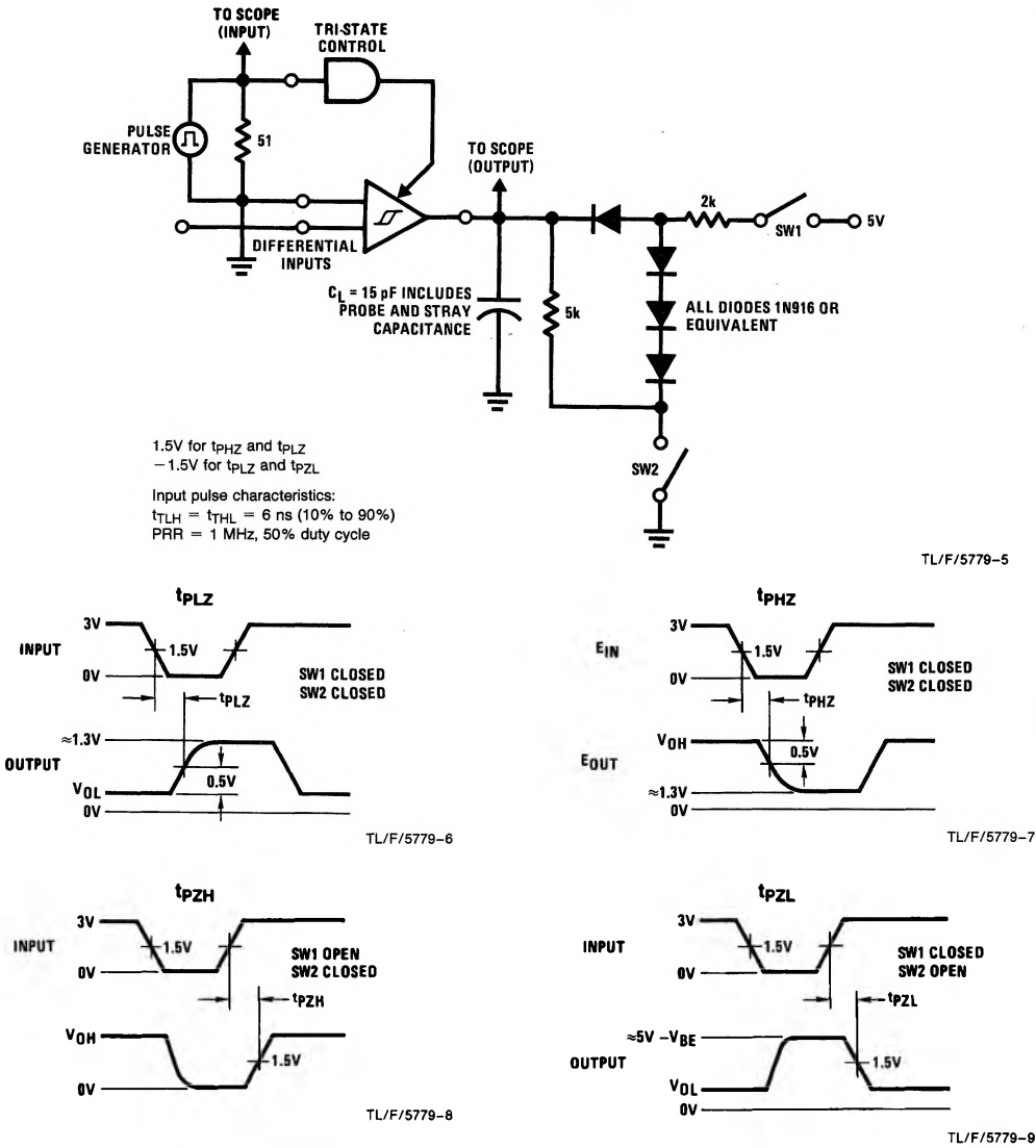
FIGURE 2. Propagation Delay TRI-STATE Control Input to Output
