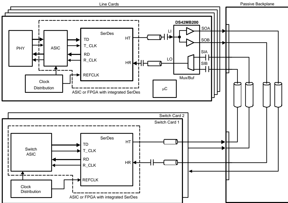
Figure 10. Application diagram (showing data paths of port 0)
