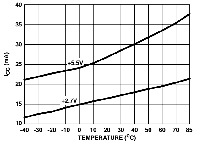
FIGURE 39. RECEIVE MODE I_{CC} vs TEMPERATURE
