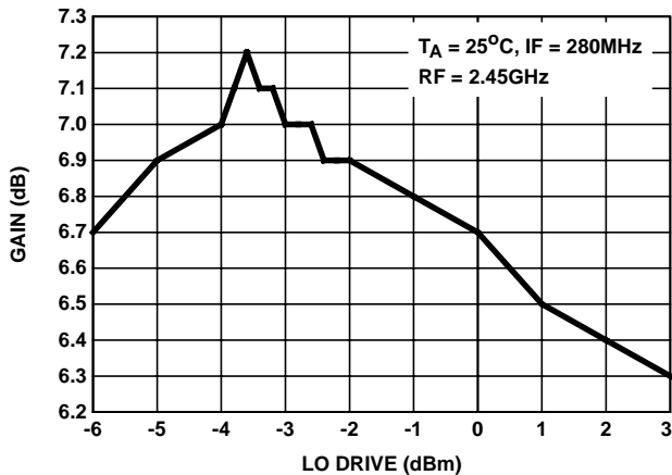
FIGURE 48. RECEIVE MIXER GAIN vs LO DRIVE
