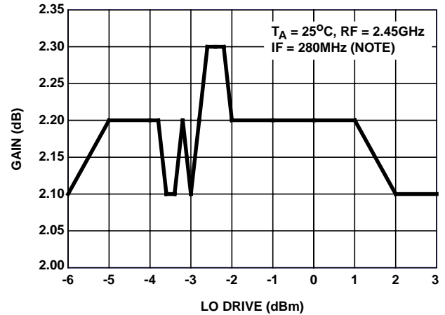
FIGURE 51. TRANSMIT MIXER GAIN vs LO DRIVE
