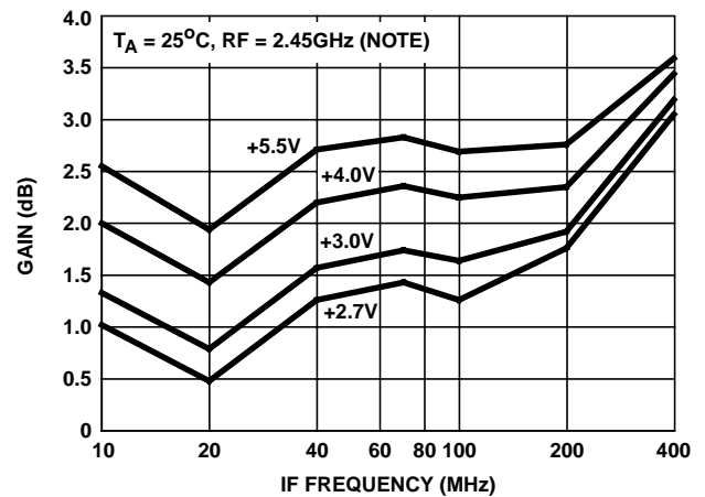
FIGURE 53. TRANSMIT MIXER GAIN vs IF FREQUENCY
