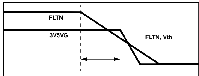
FIGURE 16. TIMING DIAGRAM
