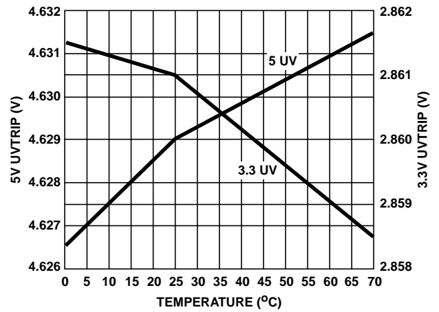
FIGURE 5. UV TRIP vs TEMPERATURE (HIP101D only)
