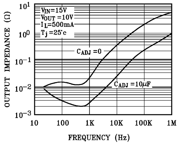
Output Impedance
