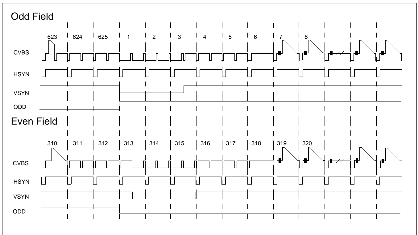
Figure 1. Synchronization Timings during Vertical Interval for 50 Hz Video
