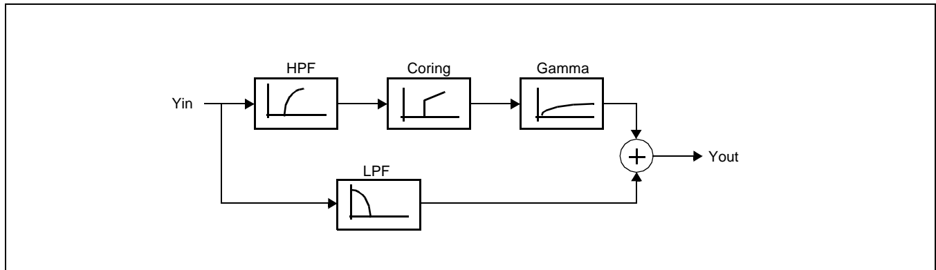
Figure 8. Cringing Circuit Block Diagram
