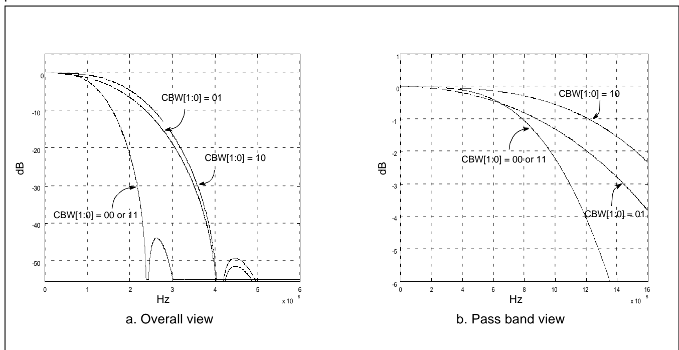
Figure 11. Chrominance Path Overall Frequency Response
