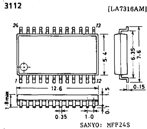
Package Dimensions (unit: mm) 3112
