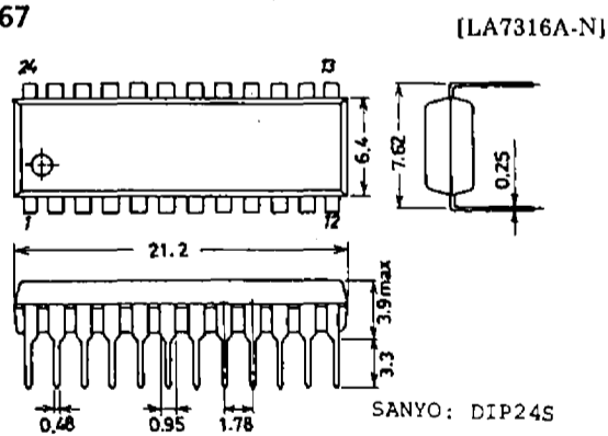
Package Dimensions ISIC (unit: mm) 3067
