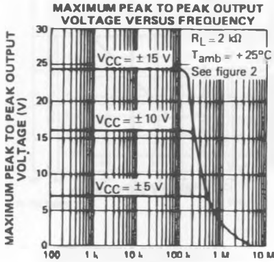
MAXIMUM PEAK TO PEAK OUTPUT VOLTAGE (V) FREQUENCY (Hz)
