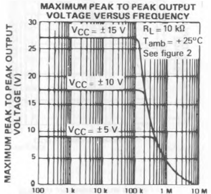
MAXIMUM PEAK TO PEAK OUTPUT VOLTAGE (V) FREQUENCY (Hz)
