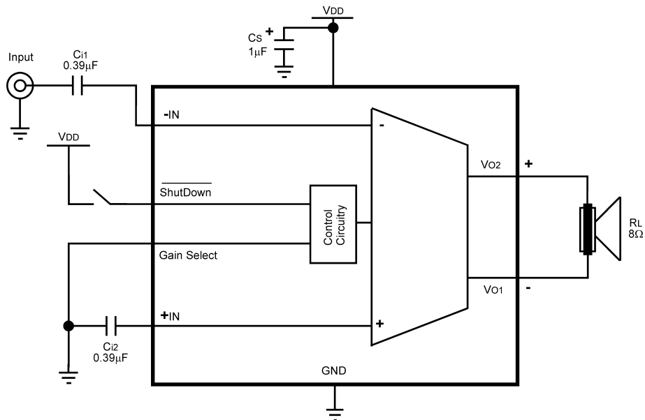
Figure 7. Single-Ended Input with high gain selection configuration
