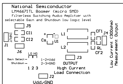
Figure 10. Top Layer
