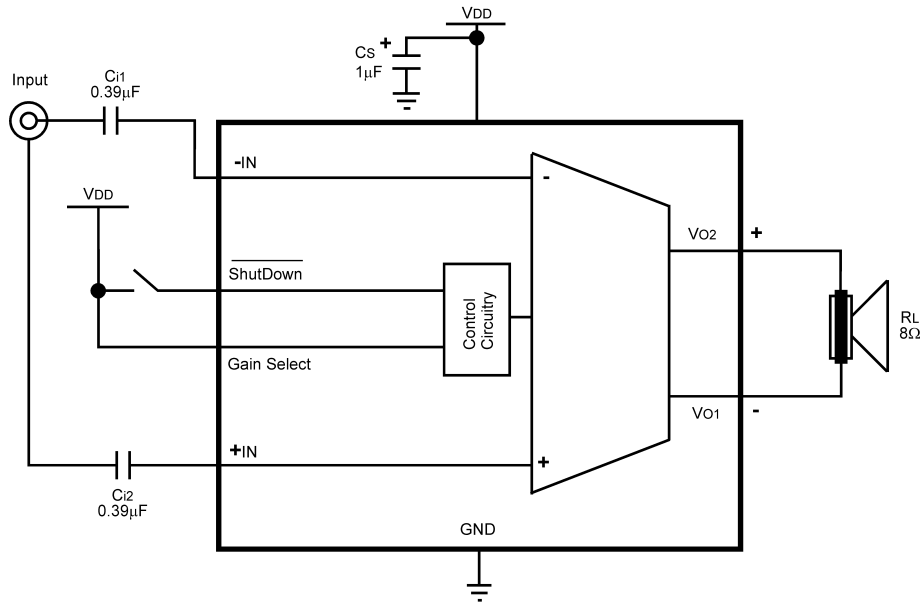
Figure 6. Single-Ended Input with low gain selection configuration
