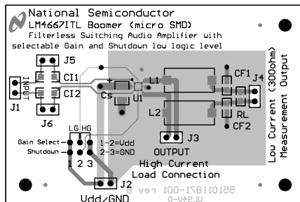
Figure 9. Silk Screen
