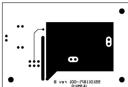
Figure 11. Bottom Layer
