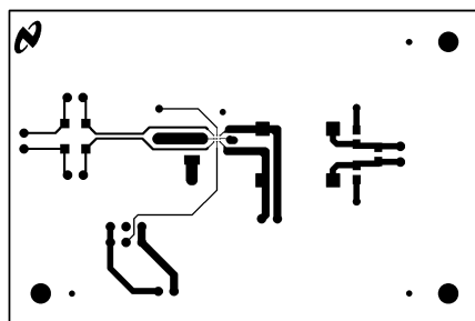
Figure 10. Top Layer
