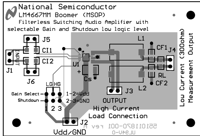
Figure 13. Silk Screen
