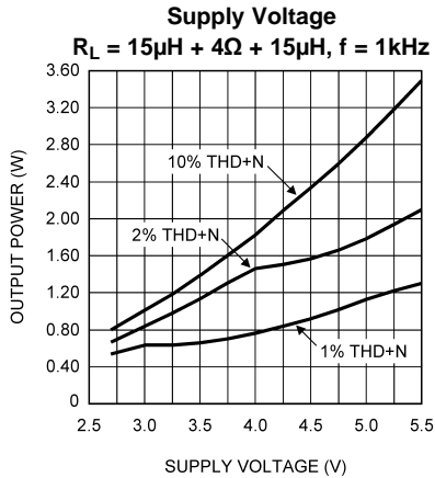
Output Power vs Supply Voltage
