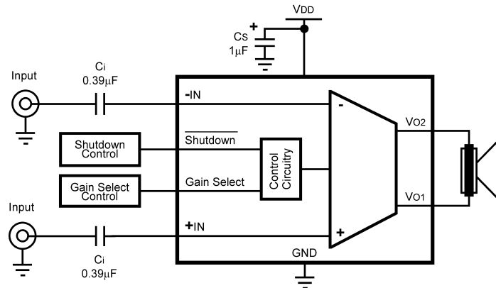
Figure 1. Typical Audio Amplifier Application Circuit
