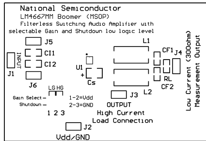
Figure 14. Top Layer
