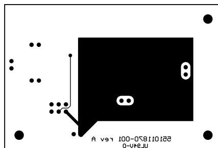
Figure 15. Bottom Layer
