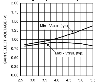
Gain Select Threshold vs Supply Voltage
