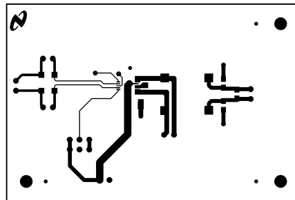
Figure 15. Bottom Layer
