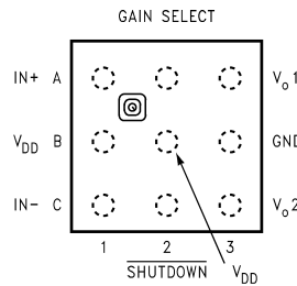
Figure 2. Top View Order Number LM4667ITL, LM4667ITLX See NS Package Number TLA09AAA
