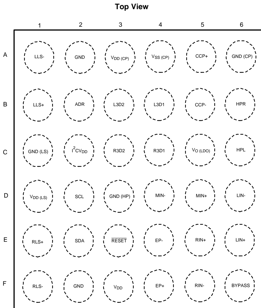
Figure 2. DSBGA Package See Package Number YPG0036CCA
