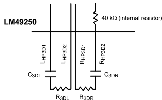
Figure 53. External 3D Effect Capacitors
