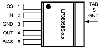
Figure 1. TO263–5, Top View
