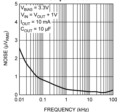
Output Noise
