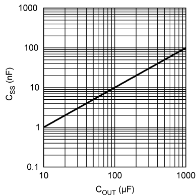
Figure 3. Typical C SS vs C OUT Values
