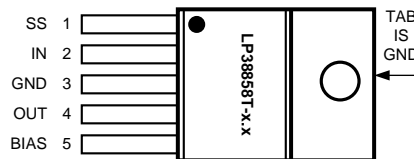
Figure 2. TO220–5, Top View
