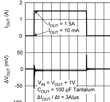
Load Transient Response, C_{OUT} = 100\ \mu\text{F} Tantalum
