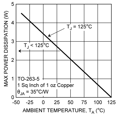
Figure 5. Maximum power dissipation vs ambient temperature for the TO-263 package
