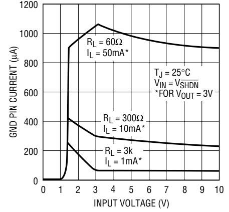
LT1763-3 GND Pin Current
