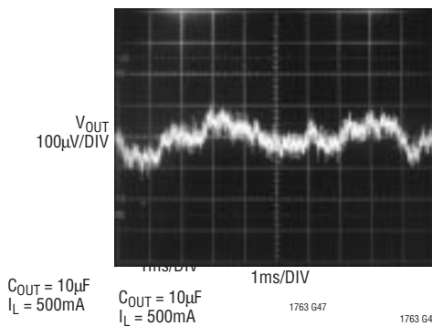
LT1763-5 10Hz to 100kHz Output Noise C_{BYP} = 1000\text{pF}
