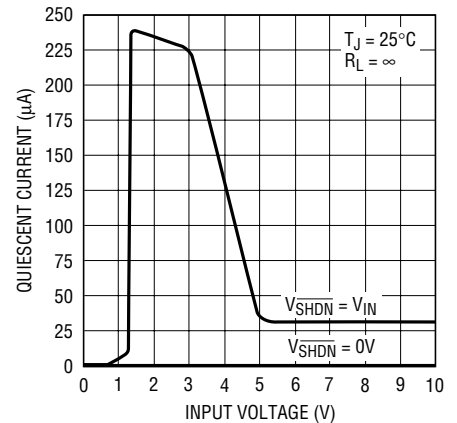
LT1763-5 Quiescent Current
