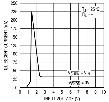
LT1763-2.5 Quiescent Current
