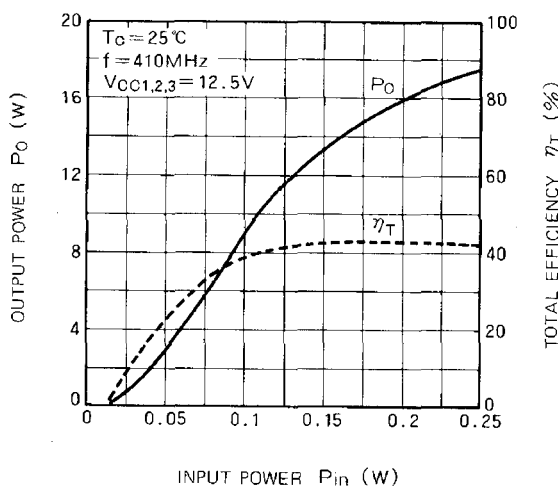
OUTPUT POWER TOTAL EFFICIENCY VS. INPUT POWER
