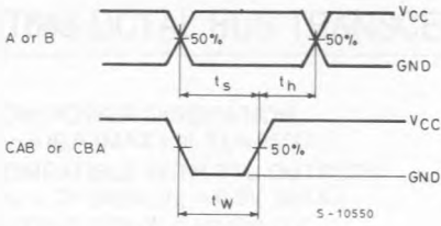
WAVEFORM 3
