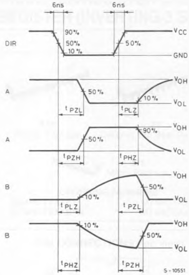
WAVEFORM 5
