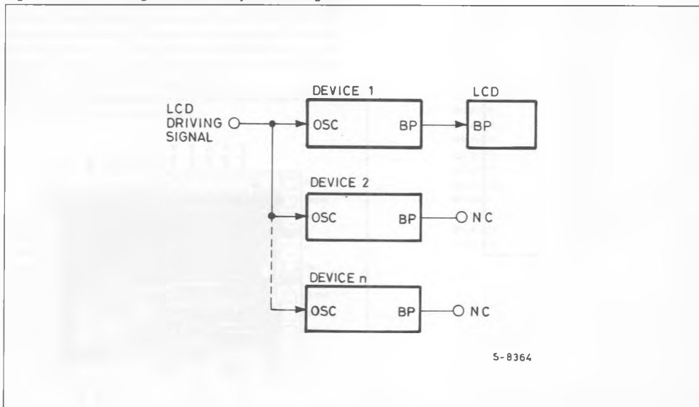
Fig. 6 - Cascade configuration, drive by external signal
