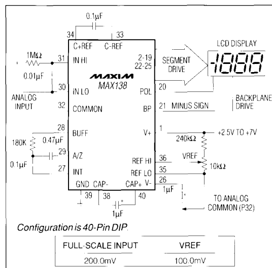
Figure 1. MAX138 Typical Operating Circuit
