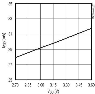
ANALOG SUPPLY CURRENT vs. ANALOG SUPPLY VOLTAGE
