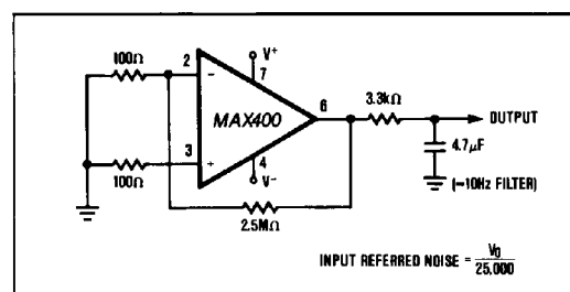
Figure 2. Low Frequency Noise Test Circuit.
