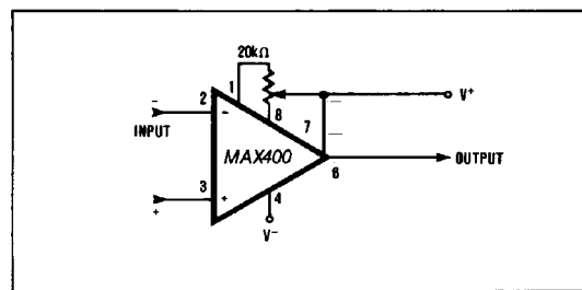
Figure 1. Optional Offset Nulling Circuit.
