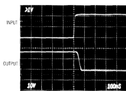
MAX4429 SWITCHING SPEED (INPUT LOW TO HIGH)
