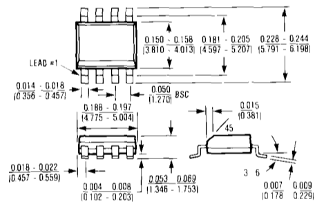
8 Lead Small Outline
