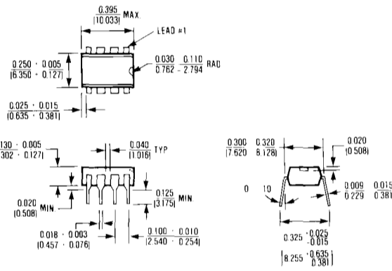
8 Lead Plastic DIP
