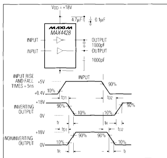
Figure 1. Inverting and Noninverting Test Circuit
