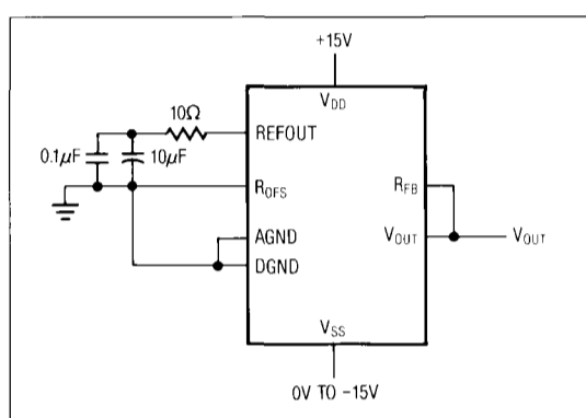
Figure 6. Unipolar Configuration (0V to +10V Output)
