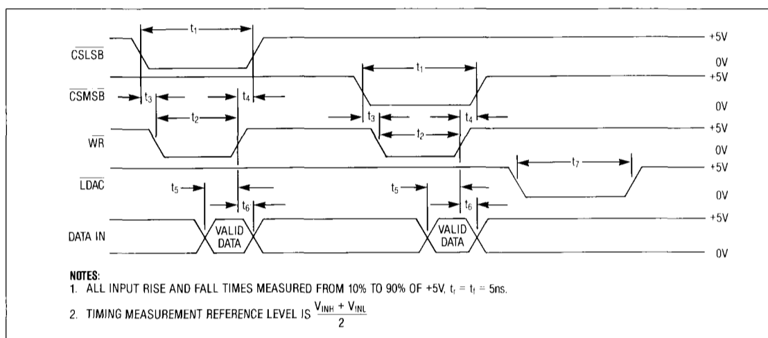
Figure 4. MAX508 Timing Diagram
