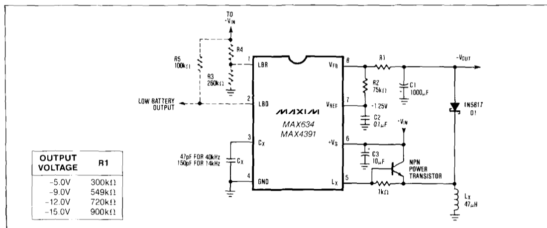
Figure 7. Boosting Output Power With External NPN Power Transistor
