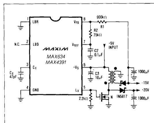
Figure 8. High Power +5V to -15V DC-DC Converter
