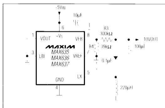
Figure 3 Adjustable Output Operation
