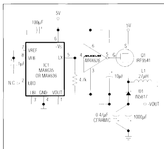
Figure 4. Medium Power Inverter
