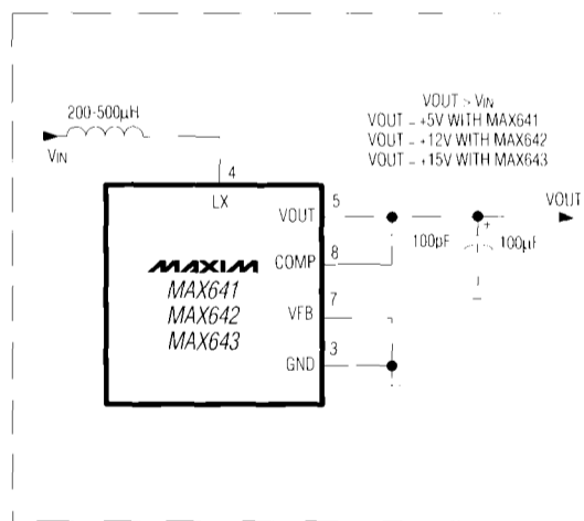
Figure 3. Low-Power, Fixed Output Step-Up Converter Using LX
