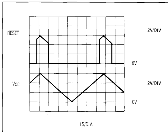
Figure 4. Typical MAX700/701/702 RESE' Output vs. Vcc
