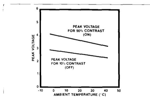
Figure 9. Temperature Dependence of Liquid Crystal Threshold.
