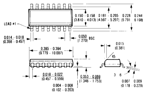
16 Lead Small Outline \theta_{JA} = 110\text{ C/W} \theta_{JC} = 60\text{ C/W}
