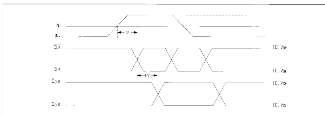
Figure 2. Timing Diagram
