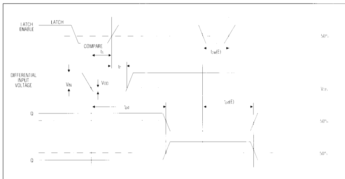
MAX9686 and MAX9698 Timing Diagram (worst case).
