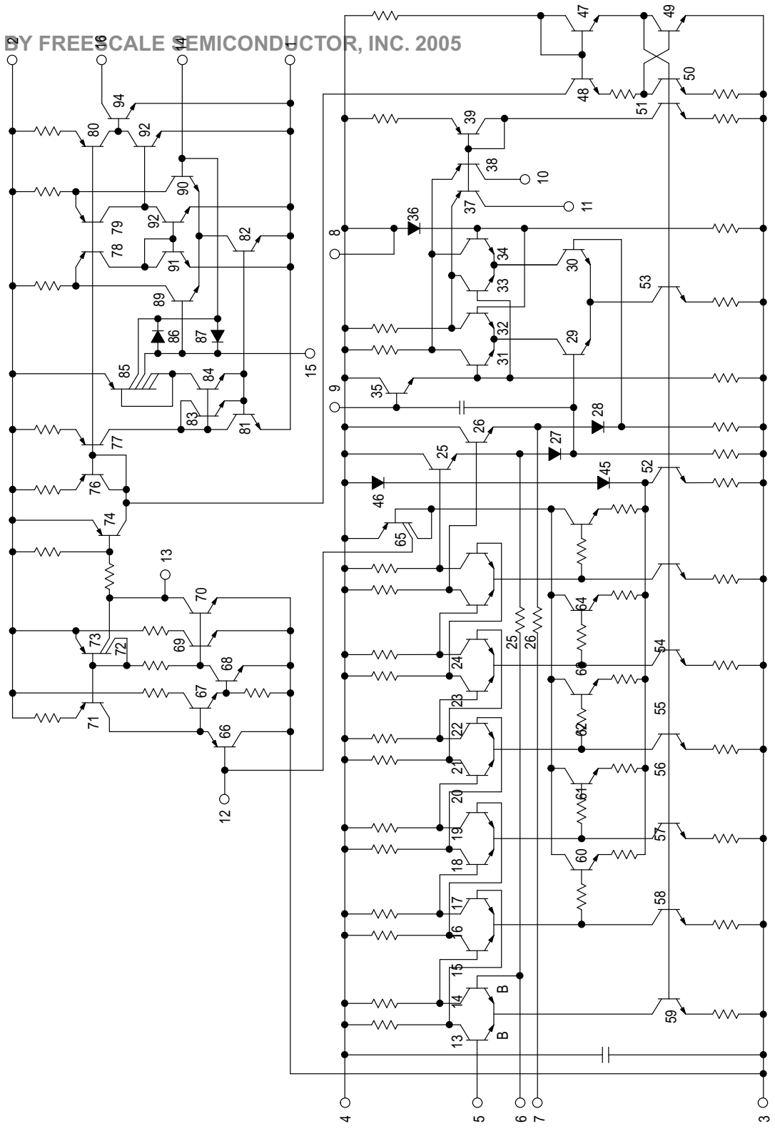
Figure 15. Internal Schematic
