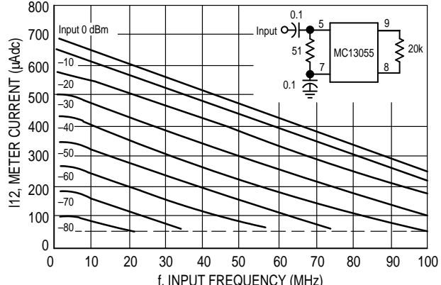
Figure 6. Untuned Input: Meter Current versus Frequency
