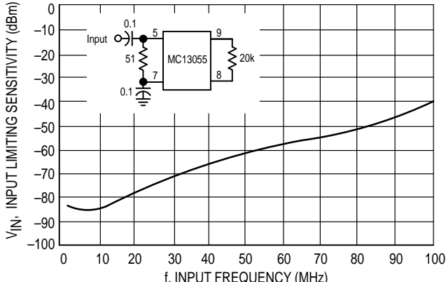
Figure 5. Untuned Input: Limiting Sensitivity versus Frequency
