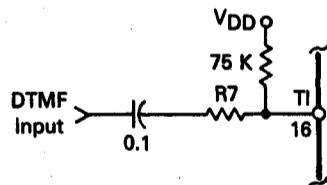
FIGURE 14 — INPUT BIASING
