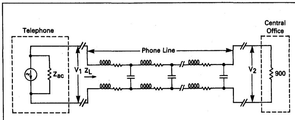
FIGURE 16 — TRANSMIT MODE
