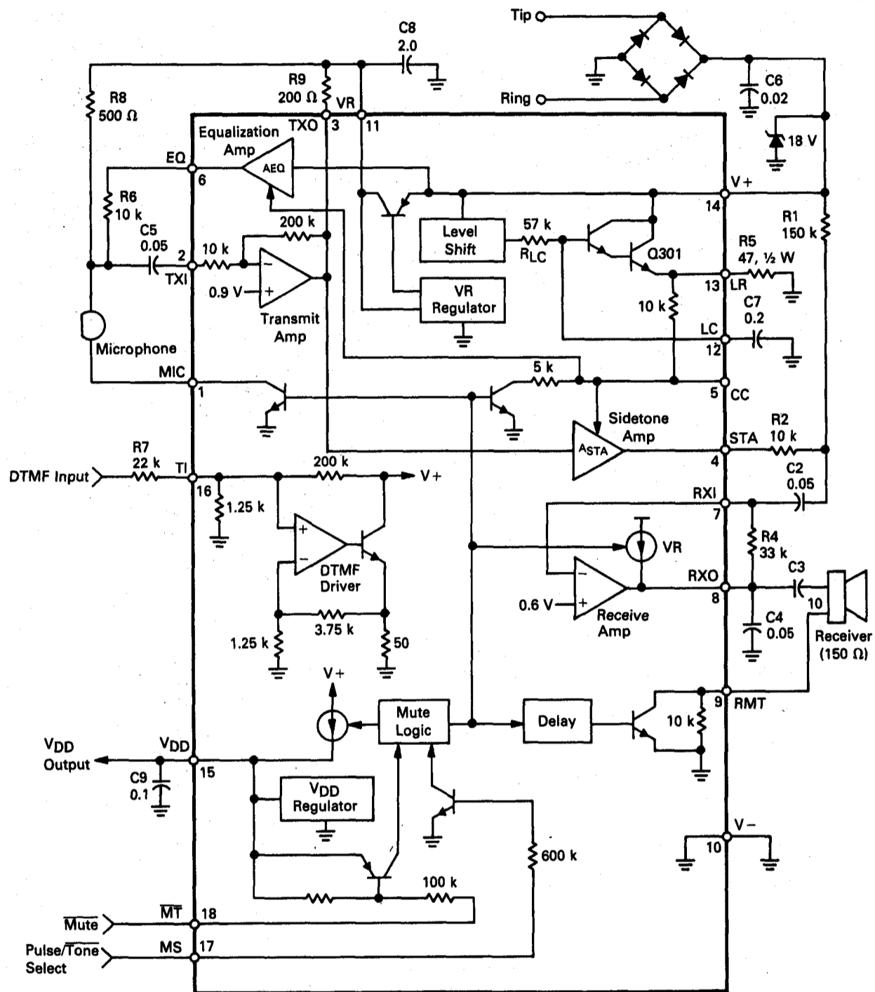
FIGURE 1 — TEST CIRCUIT
