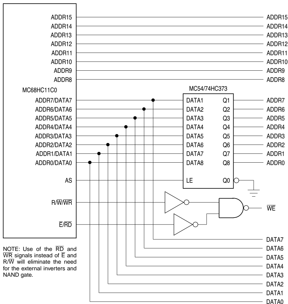
Figure 4 Address/Data Demultiplexing
