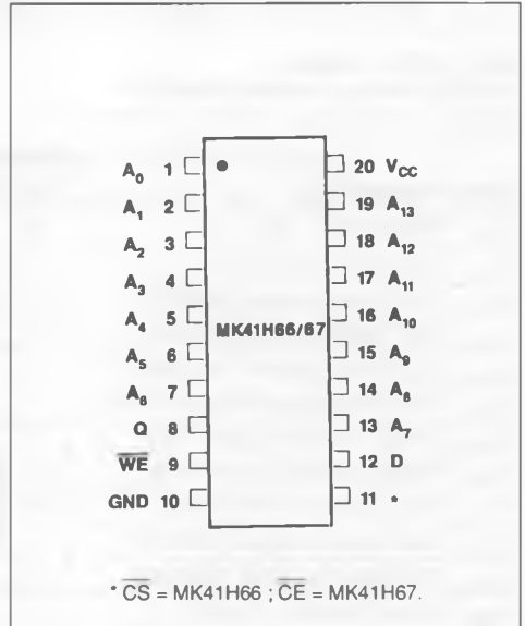
Figure 1 : Pin Connections.
