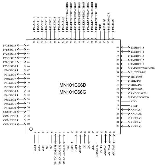
LQFP080-P-1414A *Lead-free TQFP080-P-1212D *Lead-free (under planning)
