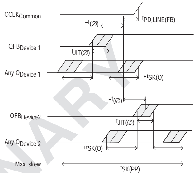
Figure 4. MPC9893 max. device-to-device skew
