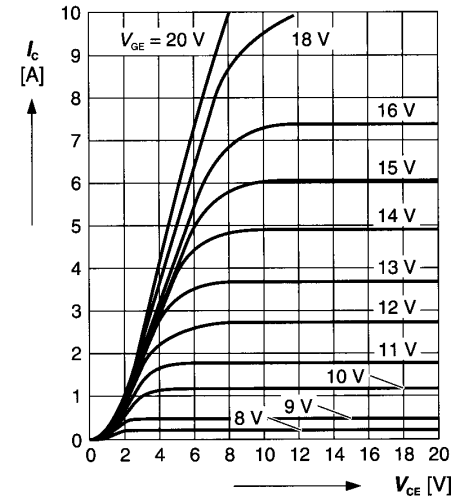
Typ. output characteristics
