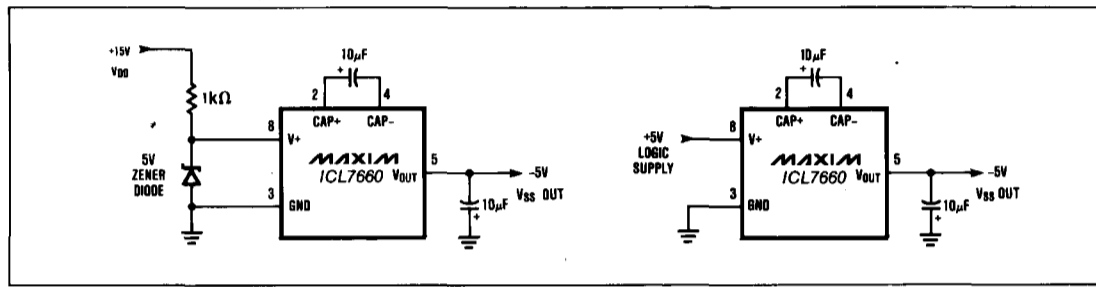
Figure 14. Generating -5V for V SS
