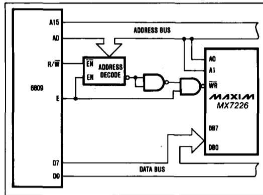
Figure 20. MX7226 to 6809 Interface
