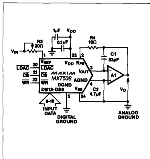
Figure 4. Unipolar Binary Operation
