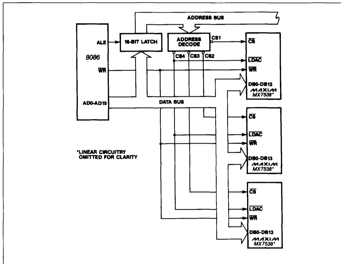
Figure 7. MX7538 - 8086 Interface: Multiple DAC System
