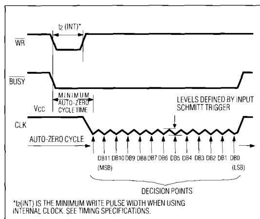
Figure 7. Operating Waveform - Internal Clock
