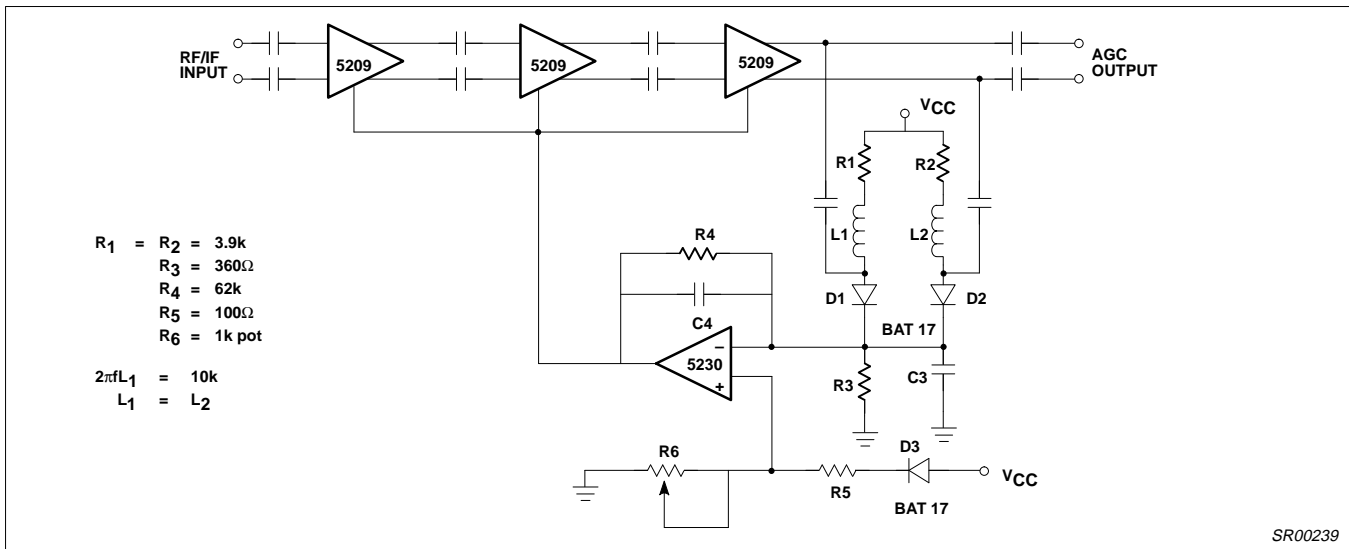
Figure 3. AGC Configuration Using Cascaded NE5209s
