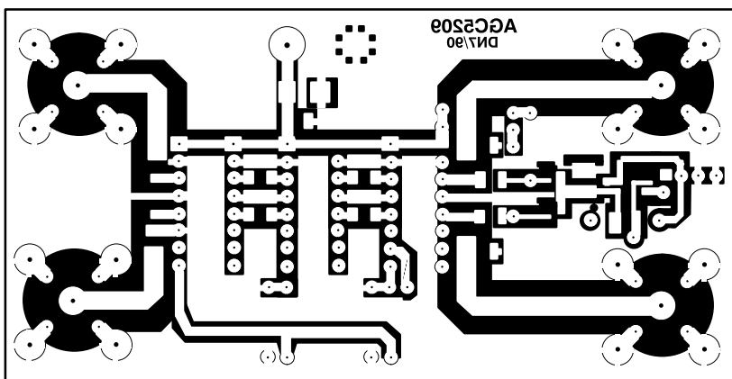
TOP VIEW - SOLDER SIDE
