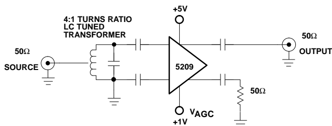
Figure 8. Narrowband Gain Optimization
