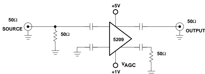
Figure 9. Simple Amplifier Configuration
