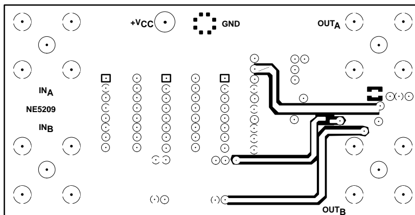
TOP VIEW - COMPONENT SIDE
