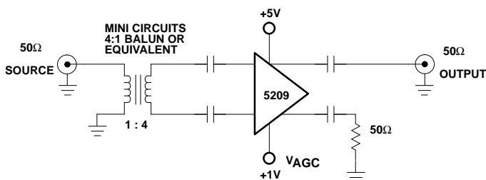
Figure 7. Broadband Gain Optimization
