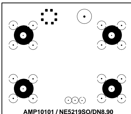
TOP VIEW - COMPONENT SIDE
