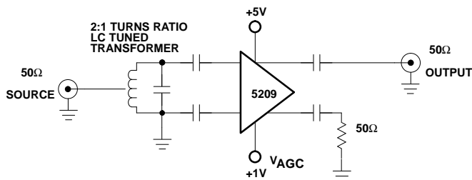
Figure 6. Narrowband Noise Optimization
