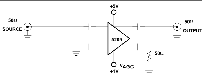
Figure 10. Underterminated Configuration
