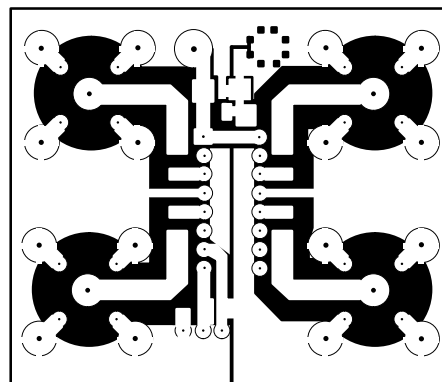
TOP VIEW - SOLDER SIDE
